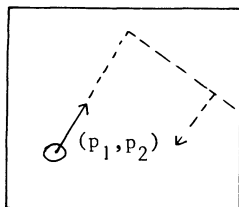
Weyl billiard
