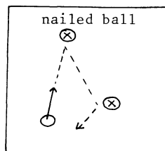
Sinai billiard
