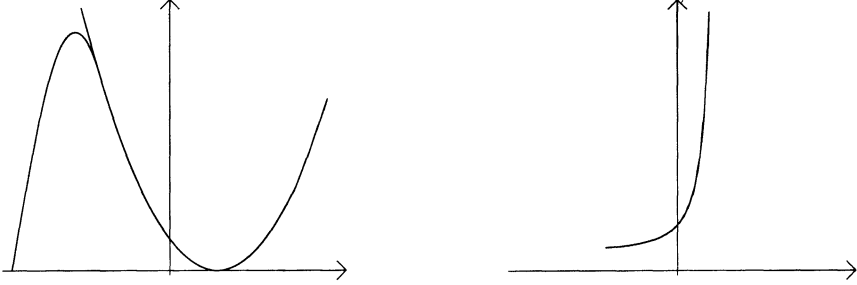
Fig. 3: b = 0.3 , e = 0 , \lambda \approx 15.42 and I \approx [-0.448, 0.3]
