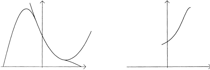
Fig. 1: b = 0.6 , e = 0 , \lambda \approx 7.13 and I \approx [-0.148, 0.548]
