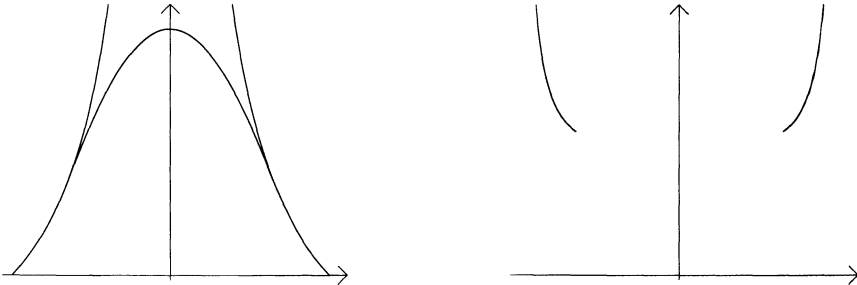
Fig. 4: \lambda_1 \approx 3.31 and I \approx [-1, -0.647] \cup [0.647, 1]
