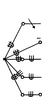
Fig. 12 - Notion d'anti-ensemble.
