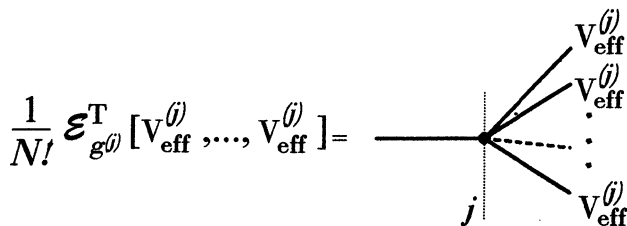
Fig. 1. Graphical representation of a truncated expectation.
