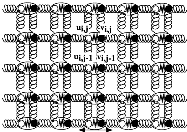
Fig. 2. – Schemes of Model 1 in two dimensions.
