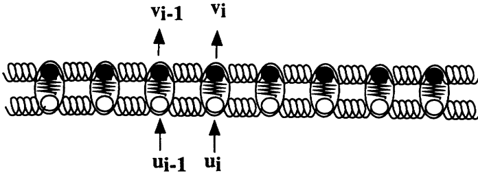
Fig. 3. – Scheme of Model 2 in one dimension.
