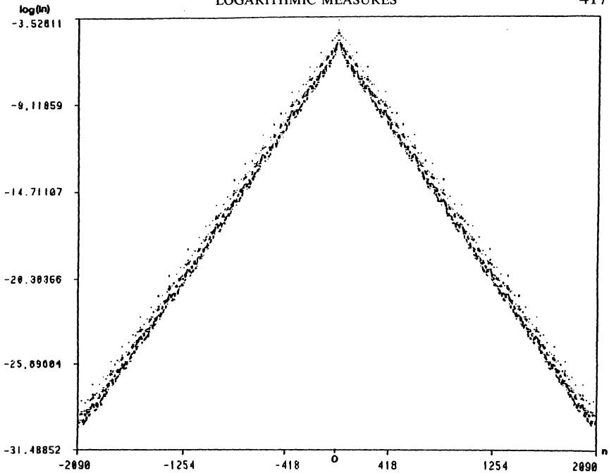
Gap structure in a cantor set of the standard map for k=0.981,635,406 , \rho=(\sqrt{5}-1)/2 . (Obtained from the rational approximation \rho'=\frac{1,597}{4,181} ).
