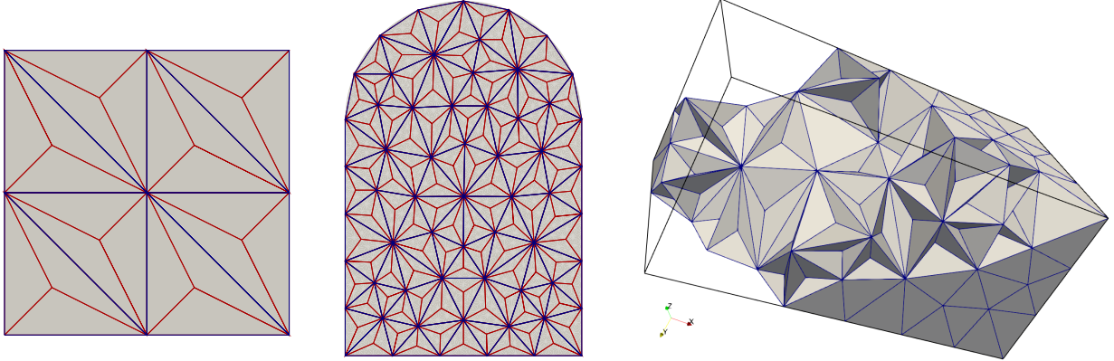
FIGURE 7.1. Example of Alfeld splits for a coarse 2D uniform mesh used in Example 1 (left), a coarse unstructured grid for Example 2 (center), and for a 3D non-uniform mesh used in Example 3 (crinkle clip on the right panel).
