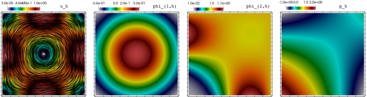
FIGURE 7.2. Example 1: Approximate velocity magnitude, temperature, concentration, and postprocessed pressure, obtained using k = 1 and a barycentrically refined mesh with 19110 elements.
