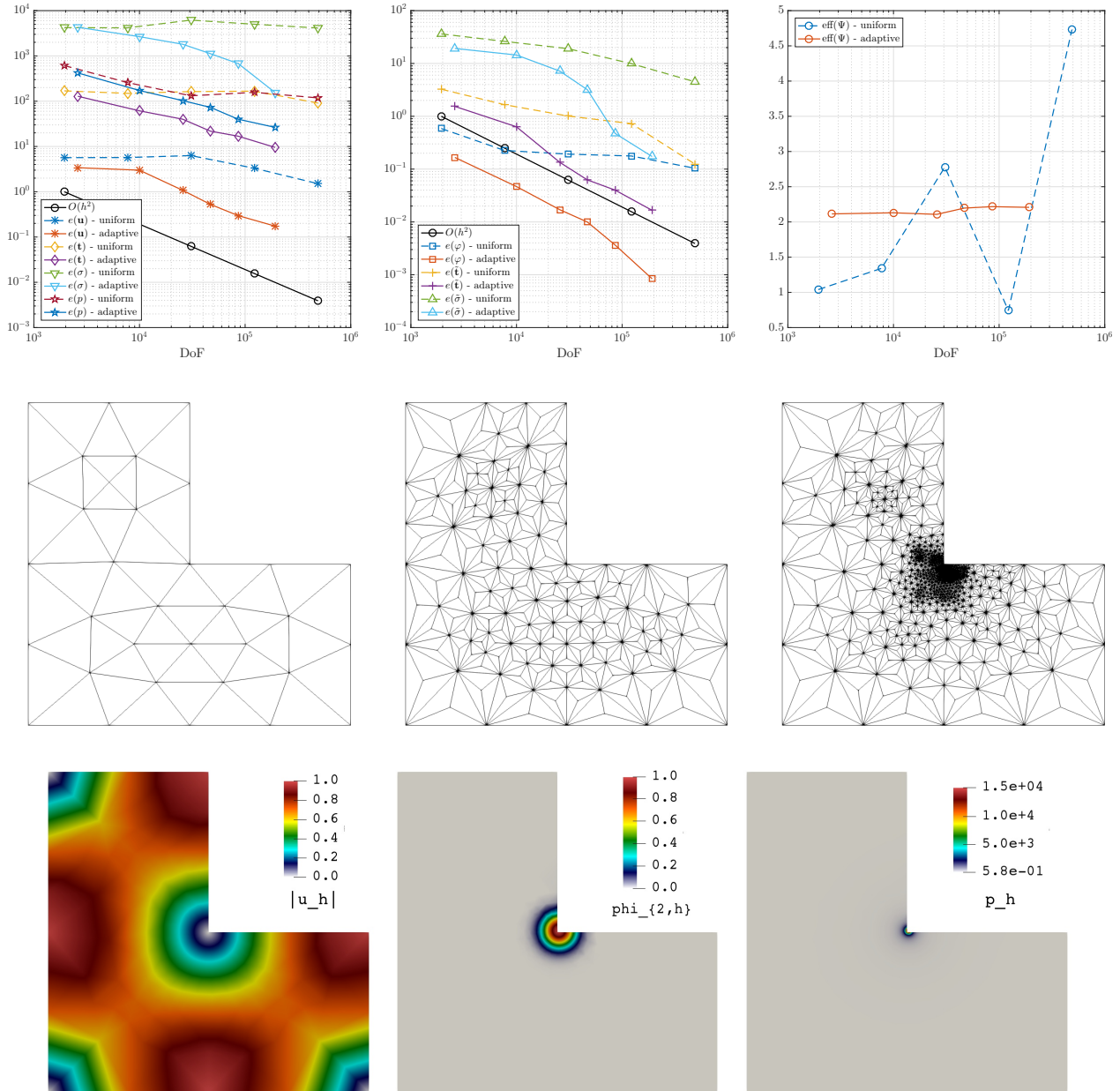
FIGURE 7.4. Example 3. Top: Error history and effectivity index for the fully-mixed method on a non-convex domain using exact solutions with high gradients and uniform vs. adaptive mesh refinement. Middle row: Initial triangulation (left) and samples of intermediate barycentric refinements obtained after three (center) and five (right) steps of mesh adaptation according to the a posteriori error estimator (6.4). Bottom panels: samples of approximate solutions on coarse adapted meshes.
