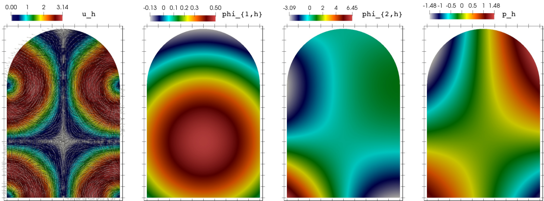
FIGURE 7.3. Example 2: Approximate velocity magnitude, temperature, concentration, and postprocessed pressure, using k = 2 and a barycentric refinement with 11534 triangular elements.
