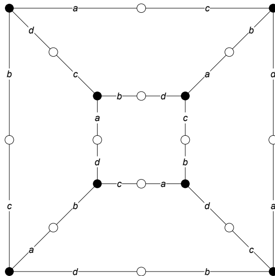
FIGURE 2.1. Schematic indication of Couveignes' dessin with parameters (a, b, c, d) based on the combinatorics of a cube. The actual dessin is obtained by replacing each \bullet \text{---} u \text{---} \circ by u parallel edges.
