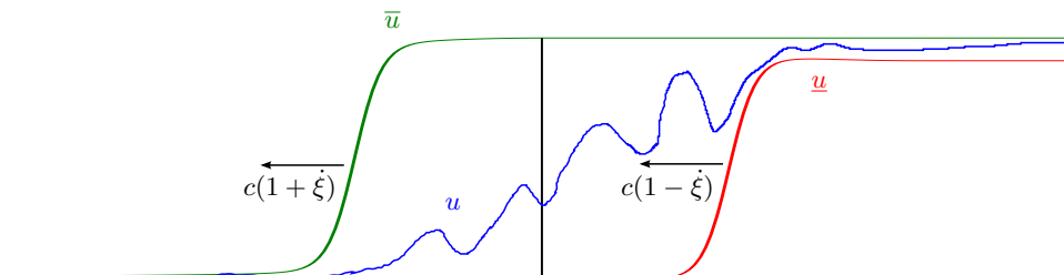
FIGURE 9. Trapping of the front-like data
