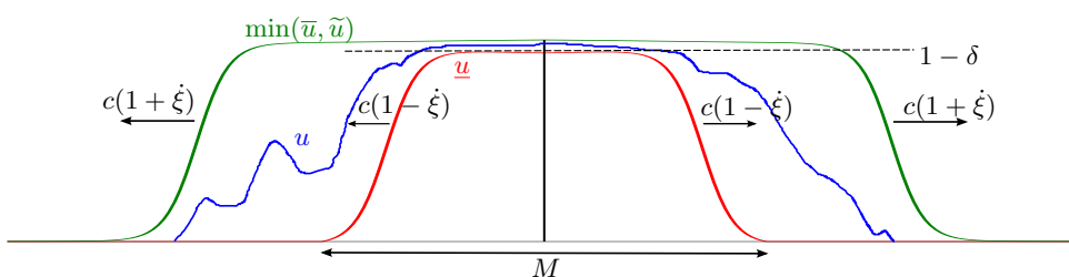
FIGURE 10. Trapping of the compactly supported data
