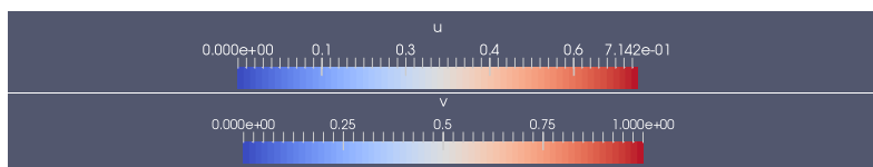
FIGURE 1. Scale. u, v are solutions of (1). u is extended in a constant way over the all \Omega_L for a clearer representation and comparison with v .
