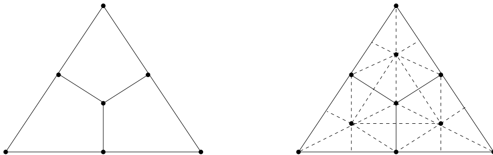
FIGURE 1. The triangulation K_3
