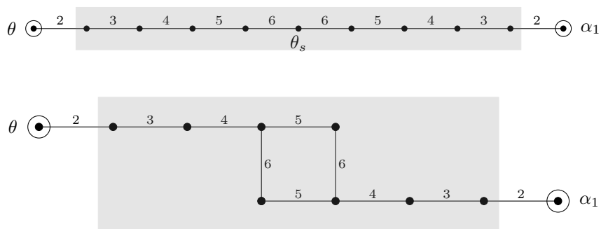
FIGURE 3. I \cong B_{6,1} and I \cong D_{6,1} . In both cases, S_I = \{\alpha_1, \theta\} . The gray boxes cover the roots in I \setminus S_I = I \cap H , with H = (\tilde{\omega}_1 - \tilde{\omega}_2)^\perp .
