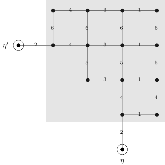
FIGURE 9. I \cong E_{7,7} , \gamma = \alpha_{\{1,3,4,5,6,7\}} . The diagram represents (\eta^{\preceq}) . The gray square covers the roots contained in H_I = (\check{\omega}_7 - \check{\omega}_2)^\perp .
