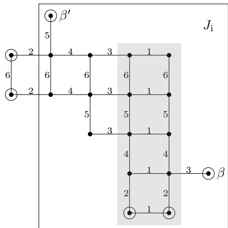
FIGURE 7. I \cong E_{7,7} , \beta = \alpha_{\{2,4,5,6,7,\}} . The gray rectangles illustrate the bipartition of (\beta^{\preccurlyeq}) . For the symmetric root \beta' = \theta - \alpha_{[1,4]} , the bipartition of (\beta'^{\preccurlyeq}) is similar.
