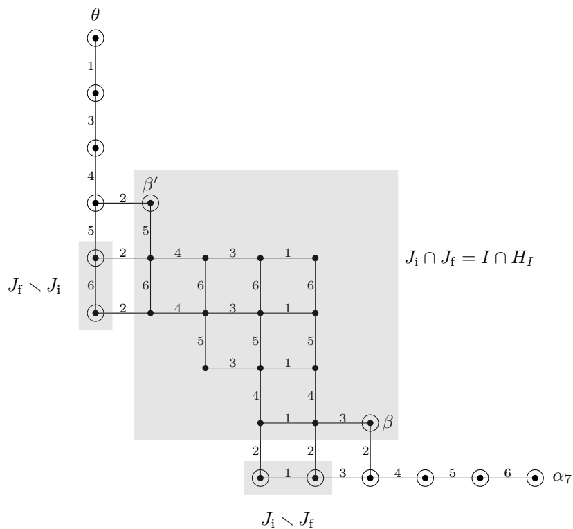
FIGURE 7. I \cong E_{7,7} , \beta = \alpha_{\{2,4,5,6,7,\}} . The gray rectangles illustrate the bipartition of (\beta^{\preccurlyeq}) . For the symmetric root \beta' = \theta - \alpha_{[1,4]} , the bipartition of (\beta'^{\preccurlyeq}) is similar.
