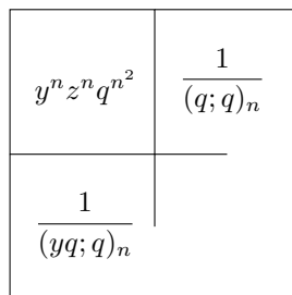
FIGURE 1. Decomposing a partition with Durfee square of length n
