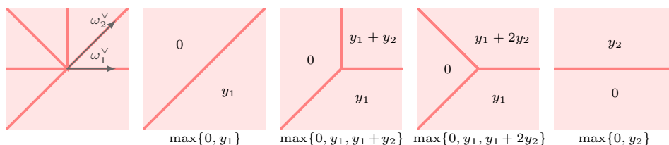
FIGURE 4. The g -vector fan of type B_2 (left) is the common refinement of the domains of linearity of the coordinate functions of \text{Trop } \Psi from Example 4.2 after intersecting with the (y_1, y_2) -plane.
