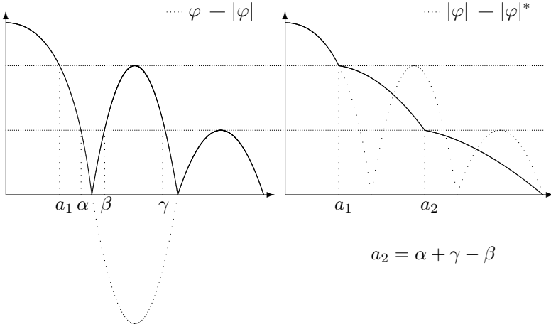
Figure 1.1. The modulus of a smooth (even) function |\varphi| and its rearrangement |\varphi|^* . Note that |\varphi|^* keeps some of the smoothness of \varphi but has a second derivative that is not in L^2 : \partial^2|\varphi|^* is of the form \psi + c_1\delta_{a_1} + c_2\delta_{a_2} . Also |\varphi|^* “oscillates” less than \varphi which means that its Fourier transform must be more concentrated near 0.
