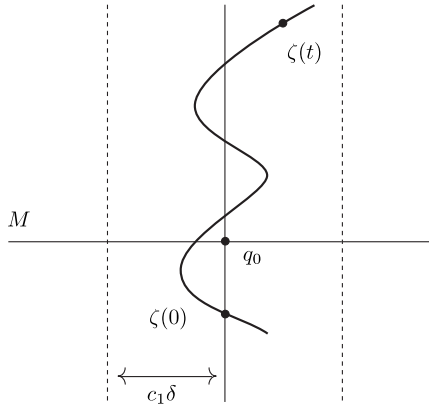
Figure 4.1. the trajectory \zeta
