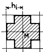
\sigma(M, 1)
