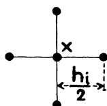
\tau(x, 1)
