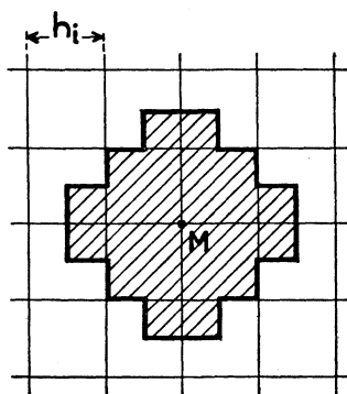
\sigma(M, 2)
