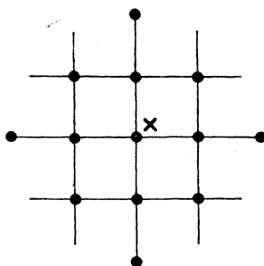
\tau(x, 2)
