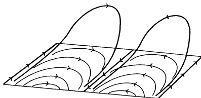
Figure 8. Orbits near Reeb component
