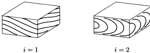
Figure 3. Basic foliations on T^2 \times I
