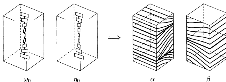
Figure 2. Projectively Anosov flow by propeller construction
