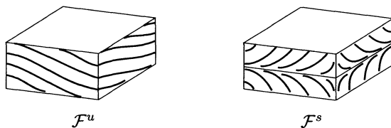
Figure 4. T^2 \times I -model
