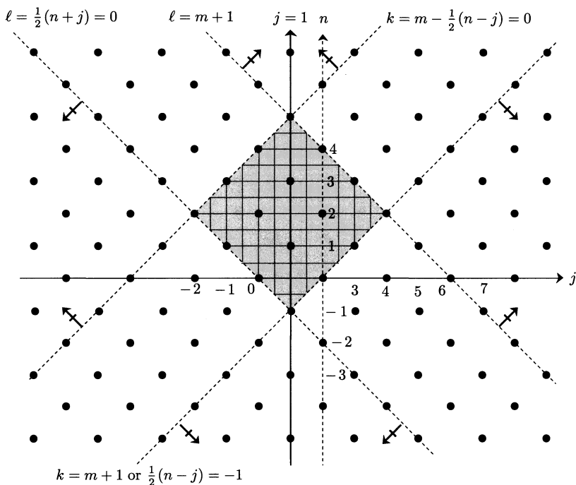
Figure 1 ( \lambda = -m = -2 ).
