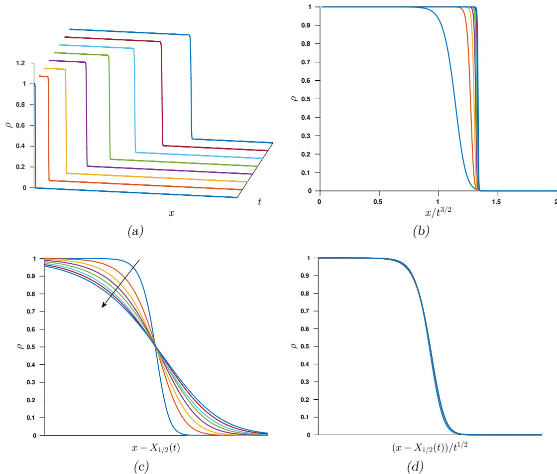
Figure A.2. Spatial propagation. (A) The numerical function \rho(t, x) is plotted for successive times at regular intervals. (B) The spatial density converges to a Heaviside function in the self-similar variable x/t^{3/2} , in agreement with the analysis performed in the article. (C) The same curves are plotted, but in the frame centered at the abscissa X_{1/2}(t) corresponding to the value \rho = 1/2 . Increasing times are figured by an arrow. The front flattens as time increases. (D) By playing with scales, I found that the typical width of the front is of order t^{1/2} , as all curves are superposed in this frame.
