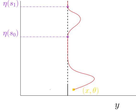
Figure 7.1. Sketch of a right D-turn between two negative times. This trajectory cannot be optimal.
