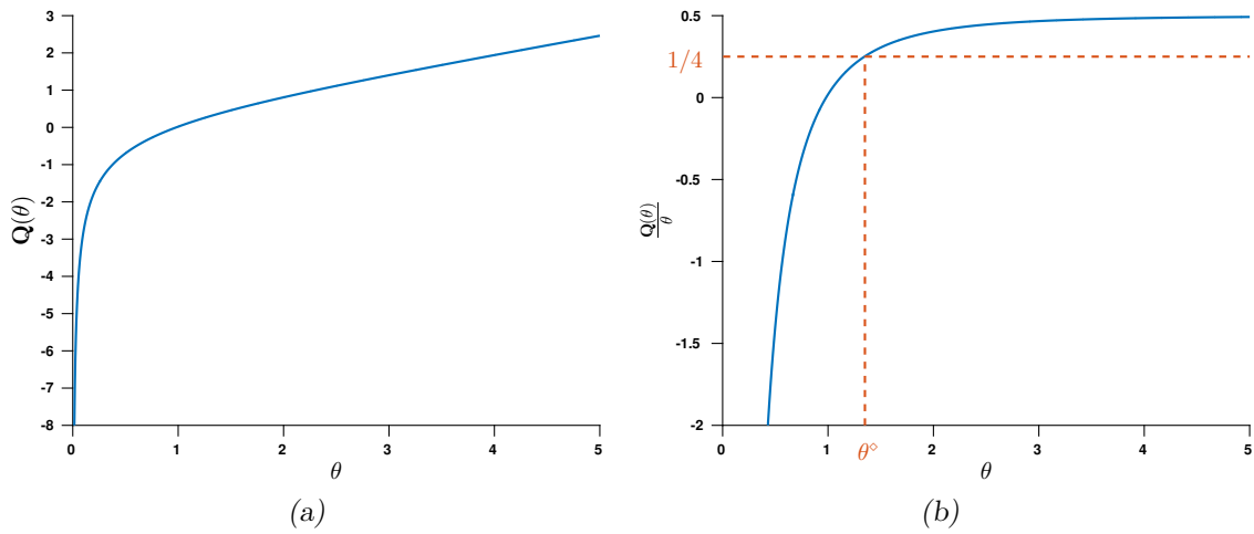
Figure 7.2. Sketch of \mathbf{Q} . Notice that both \mathbf{Q} and \mathbf{Q}(\theta)/\theta are increasing in \theta .
