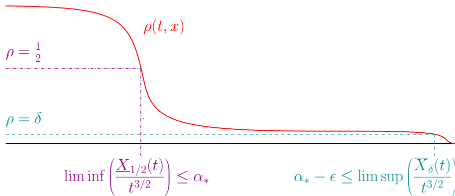
Figure 1.1. Illustration of Theorem 1.2, by means of a cartoon picture that cannot be ruled out by Theorem 1.2. The problem is to disprove the fact that different level sets may propagate at different rates.
