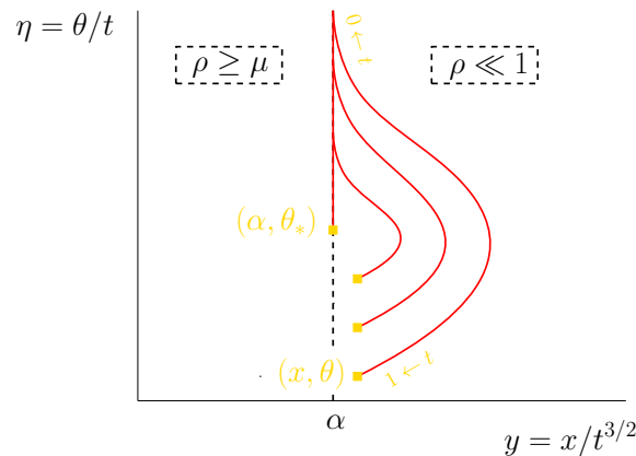
Figure 2.1. Typical optimal trajectories of (1.4) depicted in the self-similar variables plane (y, \eta) = (x/t^{3/2}, \theta/t) . The endpoint at time t = 1 is (x, \theta) . The line \{y = \alpha\} acts as a barrier due to the jump discontinuity in \rho in our argumentation by contradiction. The trajectories with endpoints on the left side of the line \{y = \alpha\} may come from the right side (not shown). However, the trajectories with endpoints on the right side never visit the left side. Moreover, for times t \rightarrow 0 , they stick to the line \{y = \alpha\} , together with \eta \rightarrow +\infty . This behavior holds true if \alpha \leq \frac{4}{3} and \mu \geq \frac{1}{2} .
