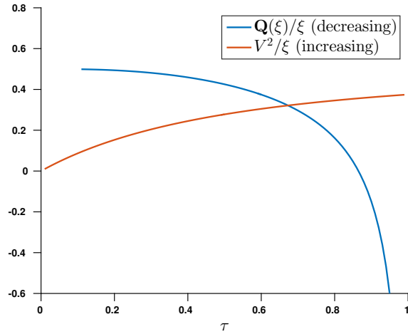
Figure 6.2. The curves \tau \mapsto \frac{Q(\xi(\tau))}{\xi(\tau)} (in blue), and \tau \mapsto \frac{V(\tau)^2}{\xi(\tau)} (in red), have a unique intersection time \tau_0 due to opposite monotonicity.
