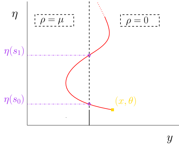
Figure 5.1. Sketch of a C-turn as the trajectory crosses the line twice. From Lemma 5.2, we see that this trajectory cannot be optimal.
