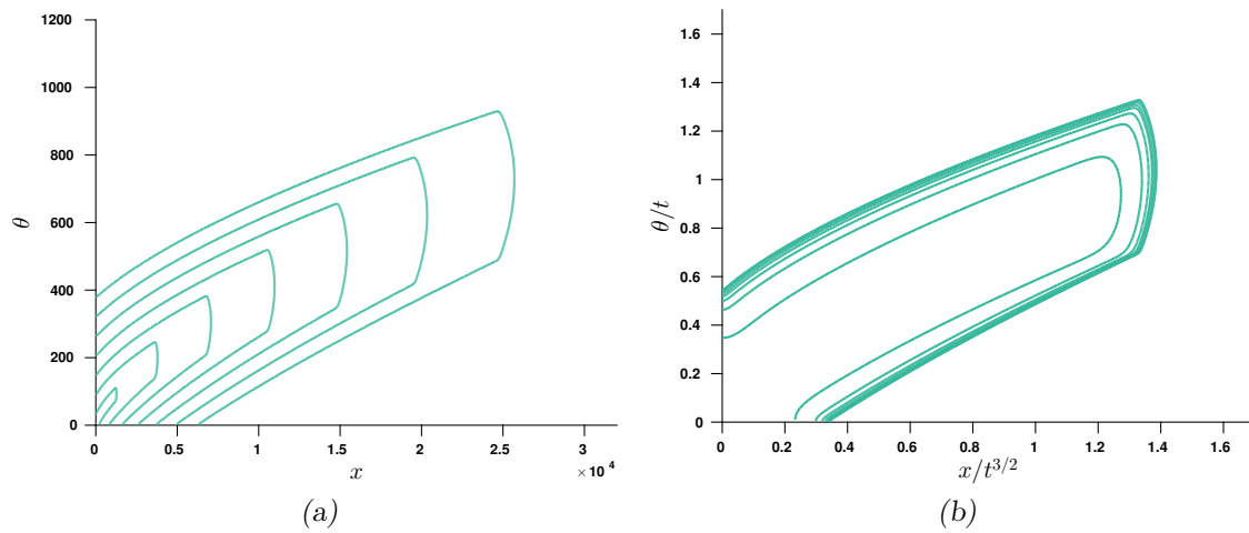
Figure A.1. One level line of the function U = -t \log f is plotted for successive times t = 100, 200, 300, 400, 500, 600, 700 with respect to the original variables (x, \theta) in (A) or with respect to the self-similar variables (x/t^{3/2}, \theta/t) in (B). One clearly sees the joint propagation in (x, \theta) towards larger x and higher \theta . Moreover, the function U seems to converge to a stationary profile in the self-similar variables, in agreement with the heuristic argument of Section 2 that u_h \rightarrow u where u_h is given by (2.1), u solves (2.2), and u and U are connected by a change of variables as in Section 4.3.
