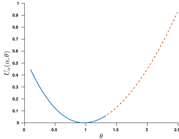
Figure 6.3. The function \theta \mapsto U_\alpha(\alpha, \theta) for the critical value \alpha = \alpha^* . The portion of the curve where s_+(\theta) < 0 is in plain line, whereas the portion where s_+(\theta) = 0 is in dashed line, that is \theta \geq \theta^\circ .
