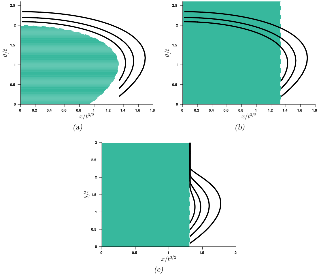
Figure 2.2. Illustration of the hindering phenomenon. The green shaded area represents the saturation zone, and the bold lines represent a sampling of optimal trajectories ending beyond the saturation zone. (A) In the case of a local saturation, that is, when f(1 - \rho) is replaced by f(1 - f) in (1.2), the saturation zone \{f \geq \delta\} , for a small \delta > 0 , is genuinely a curved area in the phase plane (x/t^{3/2}, \theta/t) . The optimal trajectories associated with (1.4) without saturation ( \mu = 0 ) are curved in a similar way. It can be shown that they do not intersect the saturation zone if their endpoint is outside the saturation zone [BHR17b, BMR15]. (B) In the case of a non-local saturation, the saturation zone \{\rho \geq \delta\} is a strip along the vertical direction. The main observation is that the optimal trajectories without saturation ( \mu = 0 ) intersect the saturation zone. This yields a contradiction as they are computed by ignoring the effect of saturation. (C) The optimal trajectories of the nonlocal problem with high enough saturation ( \mu \geq 1/2 ) do not intersect the saturation zone. Instead, they stick to the interface for some interval of time. The discrepancy between the “local” trajectories (A) and the “non-local” trajectories (C) induces a change in the value function U_\alpha , which itself is responsible for the lowering of the critical value from 4/3 (in the local version) to \alpha^* \approx 1.315 (in the non-local version).
