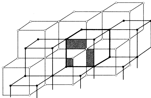
Figure 2. We have represented a complex \Sigma_0 , in full lines, with a fundamental domain in thicker lines; \Sigma_0 has three kinds of faces, a big square and two smaller parallelograms. The translate T^3\Sigma_0 is represented in dashed lines, and the dashed area shows the intersection of a square face of \Sigma_0 with the square faces of the translate; this intersection is not connected.
