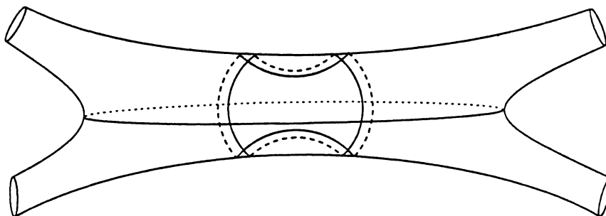
Fig. 3. — The intersection D(p_i) \cap D(p_j) has two components.
