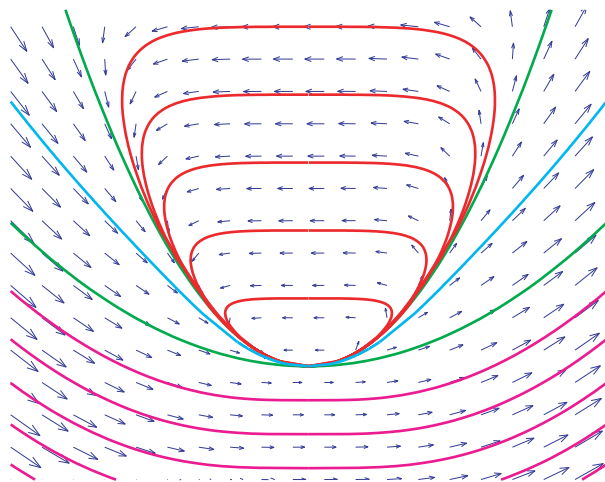
Fig. 3. A rendering, using John Polking's pplane, of orbits of (2.4).
