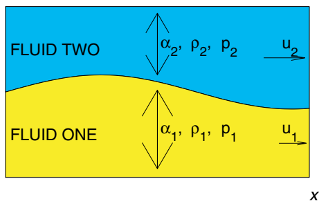
Fig. 4. Variables in the two-fluid model: Separated fluids.
