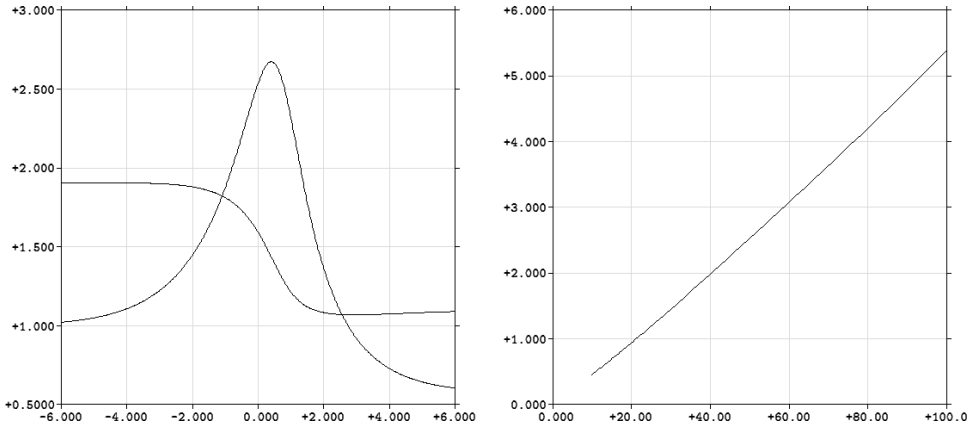
Fig. 8. Profiles of \beta and v , \epsilon = 0.05 ; \log(v^\epsilon(0)) vs. \epsilon .
