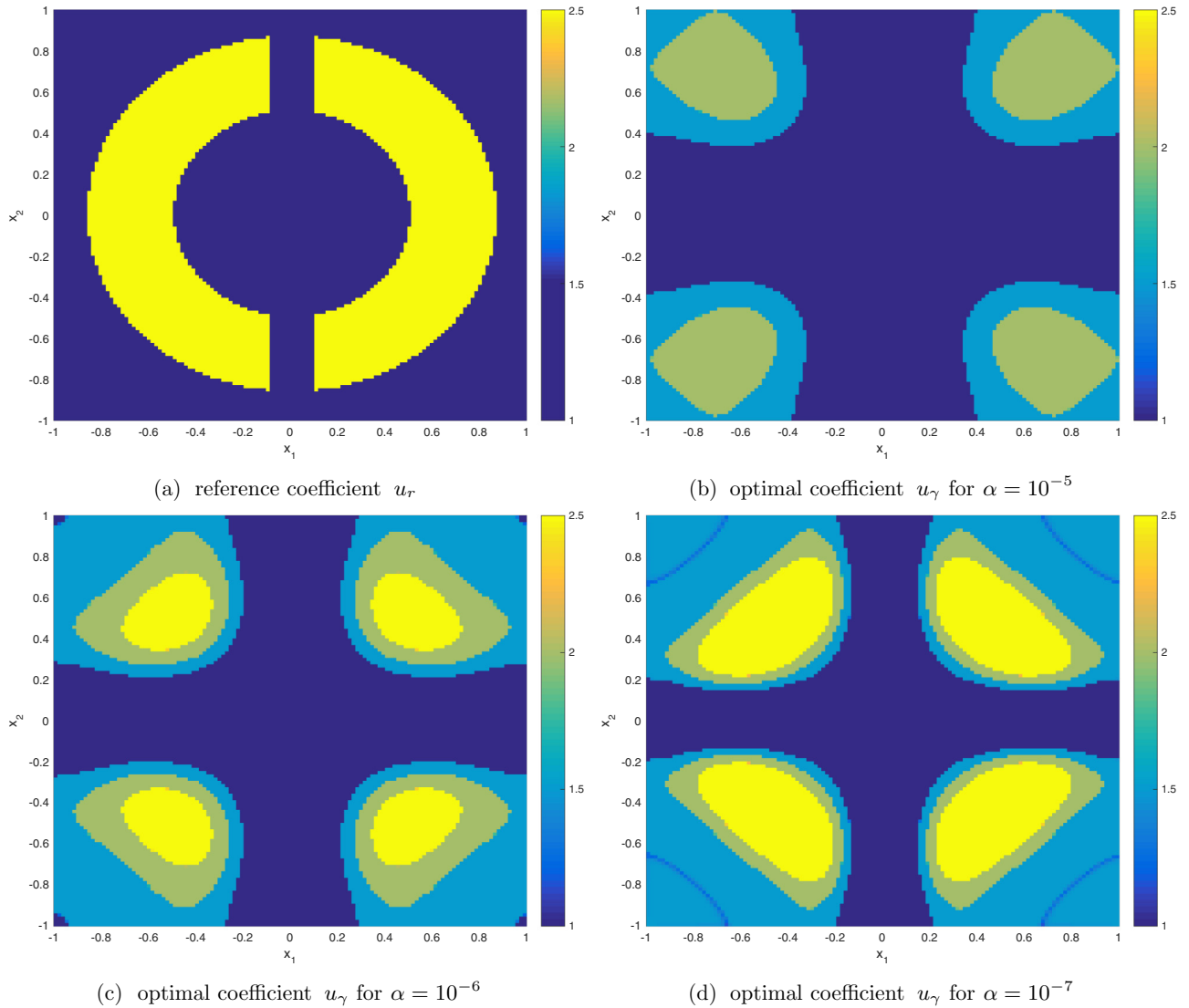
FIGURE 3. Results for potential problem.
