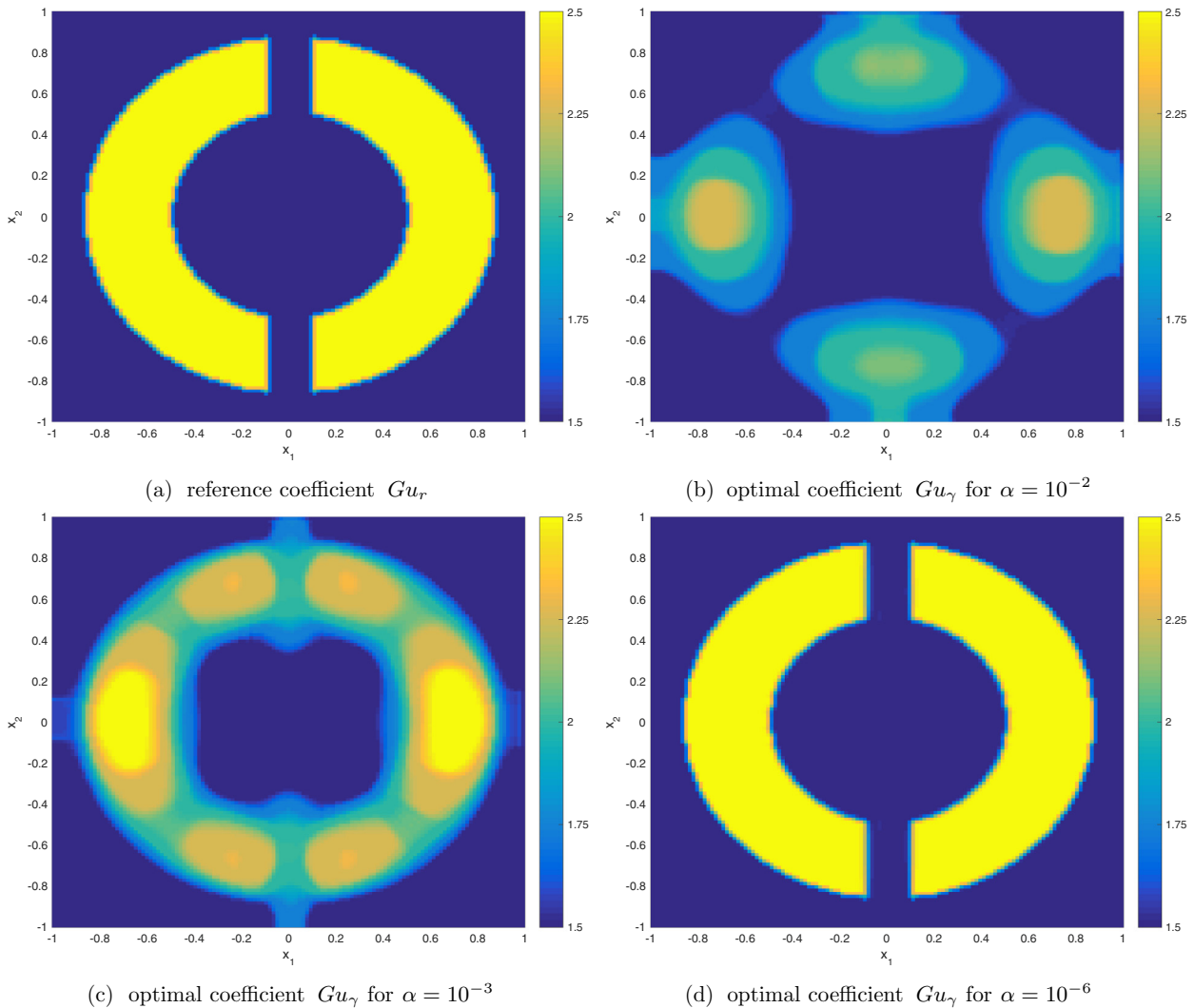
FIGURE 4. Results for diffusion problem.
