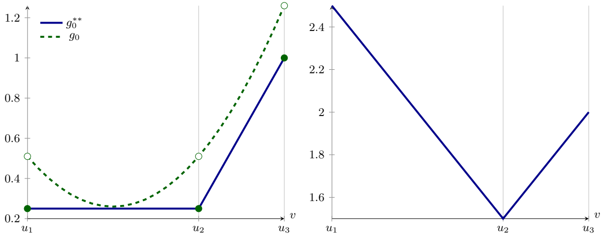
FIGURE 1. Plot of g_0^{**} and g_0 (left), h (right) for d = 3 , (u_1, u_2, u_3) , \alpha = 0.5 , \beta = 0.26 (satisfying (2.16)).
