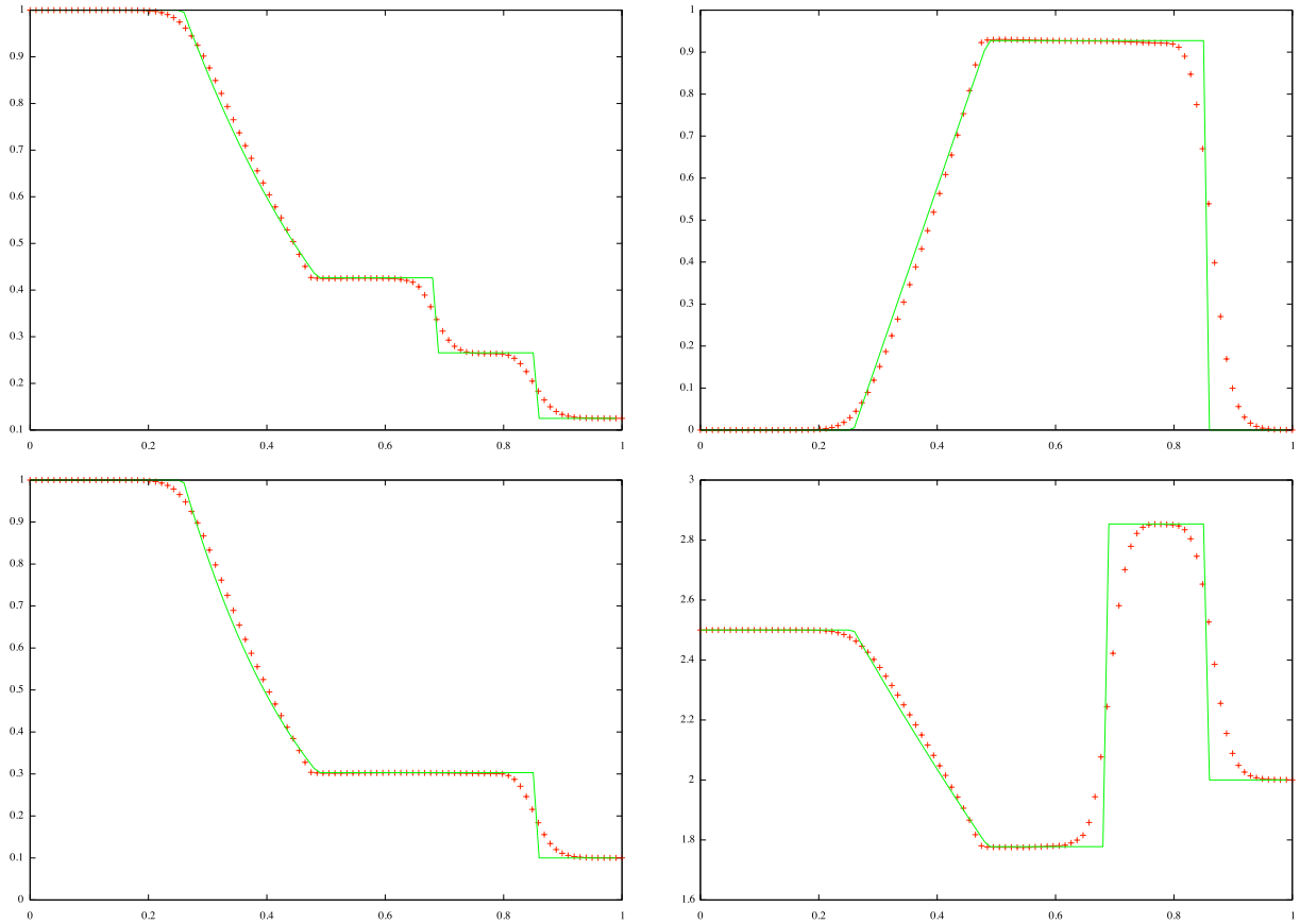
FIGURE 3. Sod shock tube, solution obtained with 100 particles compared to exact solution (solid line), from left to right and from top to bottom: density, velocity, pressure, thermal energy.
