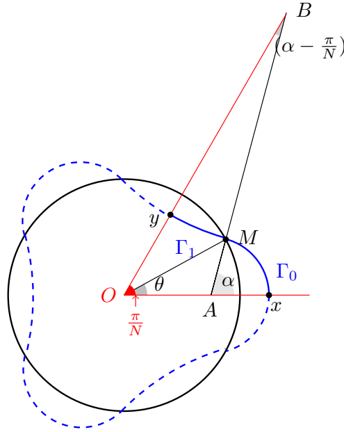
FIGURE 6. Connected case. A set \Omega with one optimal ball, N = 3 .
