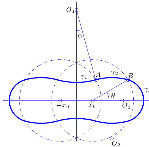
FIGURE 7. Parametrization of a mask M with \alpha, \theta, x_0 .
