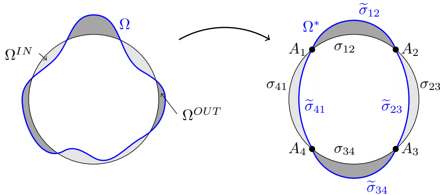
FIGURE 1. A set \Omega and its symmetrization \Omega^* .
