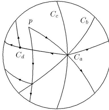
Fig. 1. Broken geodesics on \mathbb{S}^2 starting at p . Here C_a = C_b \cap C_c .
