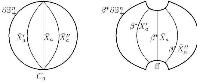
Fig. 3. The blowup of C_a in \mathbb{S}_+^n ; \beta = \beta[\mathbb{S}_+^n; C_a] is the blow-down map and \text{ff} = \beta^*C_a . X'_a and X''_a denote translates of X_a in \mathbb{R}^n , \bar{X}'_a = \text{cl}(\text{RC}(X'_a)) , etc. Note that the lifts of \bar{X}_a , \bar{X}'_a and \bar{X}''_a become disjoint on [\mathbb{S}_+^n; C_a] .
