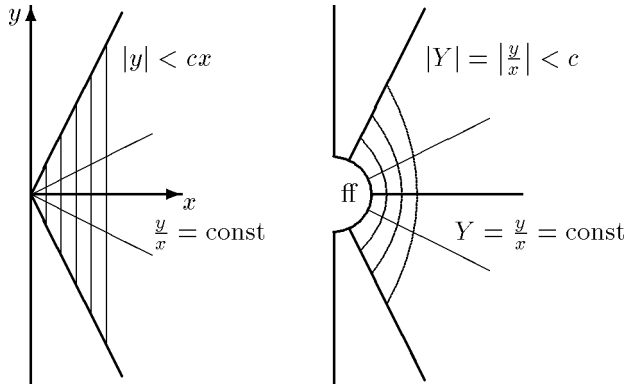
Fig. 2. The blowup of C_a = \{x = 0, y = 0\} ; the z coordinates are normal to the page and are not shown. The thin lines are the coordinate curves Y = \text{const} and x = \text{const} in the region |Y| < c (which is disjoint from \beta[X; C_a]^* \partial X ), and their images under the blow-down map \beta[X; C_a] .
