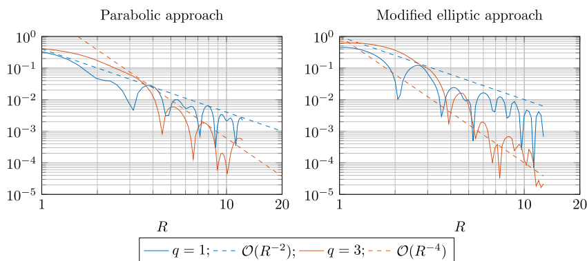
Fig. 1. Modelling error for the homogenization of the multiscale coefficients (13). Modelling parameters are k_0 = 1/2 and k_T = \frac{k_0}{\pi\sqrt{4\beta\alpha}} .
