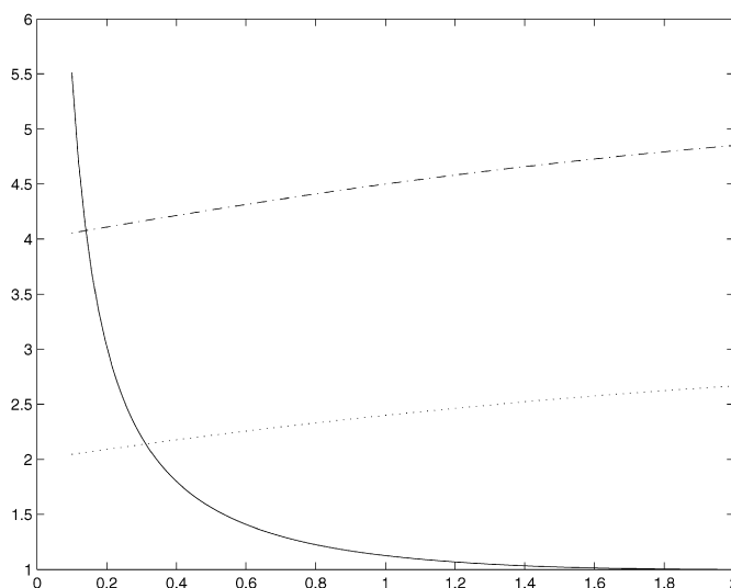
Fig. 1. Validity of (38) compared with the validity of (40). The values of \alpha lie on the horizontal axis. The continue line represents the quantity \frac{(2+\alpha)^2}{8\alpha} . The dotted line is the left-hand side of (38) and the remaining line is the left-hand side of (40).
