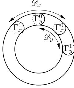
FIG. 8. — Location of the domains \mathcal{D}_x and \mathcal{D}_y on the Riemann surface \mathbf{T}
