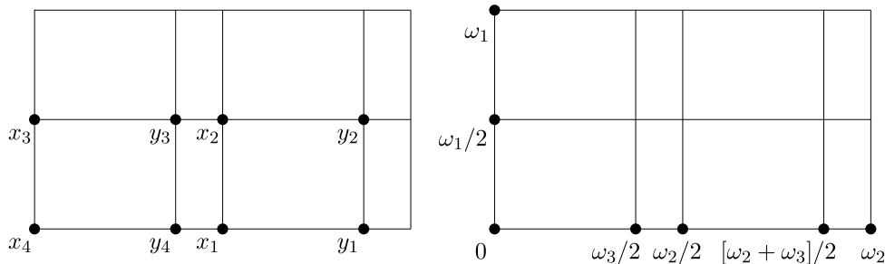
FIG. 5. — The Riemann surface \mathbf{C}/(\omega_1\mathbf{Z} + \omega_2\mathbf{Z}) and the location of the branch points
