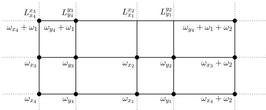
Fig. 7. — Important points and cycles on the universal covering
