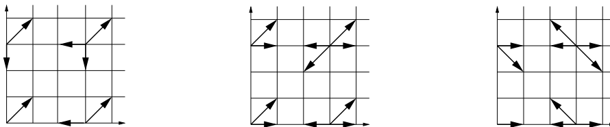
FIG. 10. — Three famous examples, known as Kreweras', Gessel's and Gouyou-Beauchamps' walks, respectively
