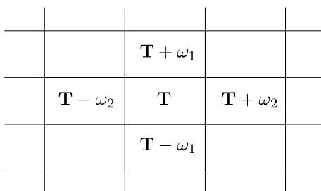
FIG. 6. — Informal construction of the universal covering
