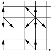
FIG. 1. — Example of model (with an infinite group) considered here—on the boundary, the jumps are the natural ones: those that would take the walk out \mathbf{Z}_+^2 are discarded
