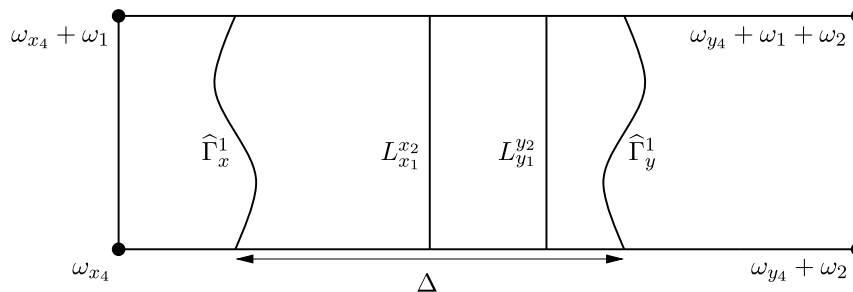
FIG. 9. — Location of \Delta = \Delta_x \cup \Delta_y
