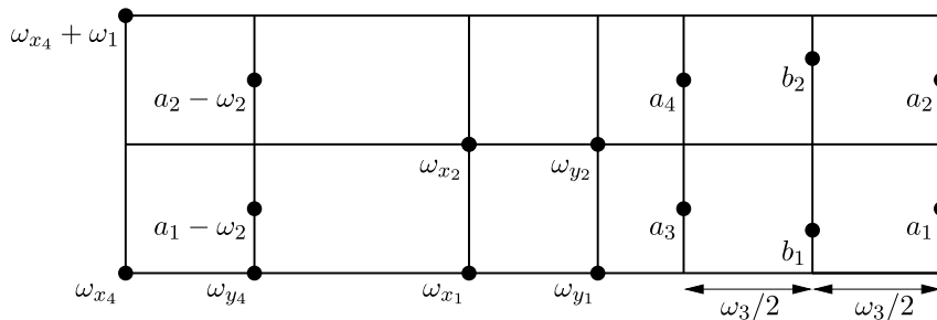
FIG. 12. — Location of a_1, a_2, a_3, a_4, b_1, b_2 if y_4 < 0 and x_4 < 0 , i.e., Subcase I.A
