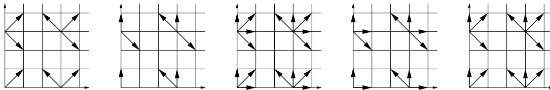
FIG. 2. — The 5 singular walks in the classification of [2]
