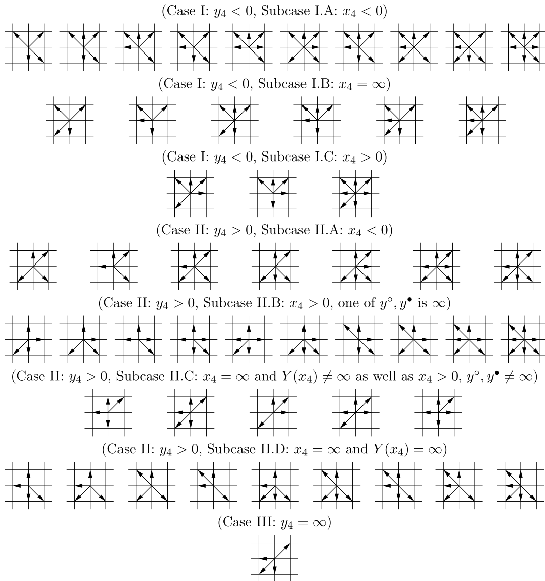
FIG. 17. — Different cases considered in the proof of Theorem 17—they correspond to the 51 non-singular walks with infinite group, see [2]
