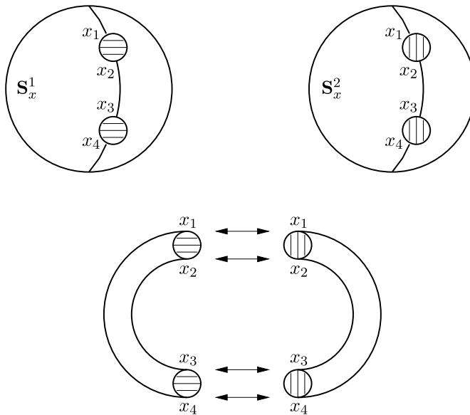
FIG. 3. — Construction of the Riemann surface
