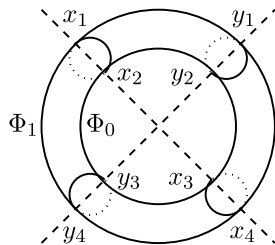
FIG. 4. — Location of the branch points and of the cycles \Phi_0 and \Phi_1 on the Riemann surface \mathbf{T}
