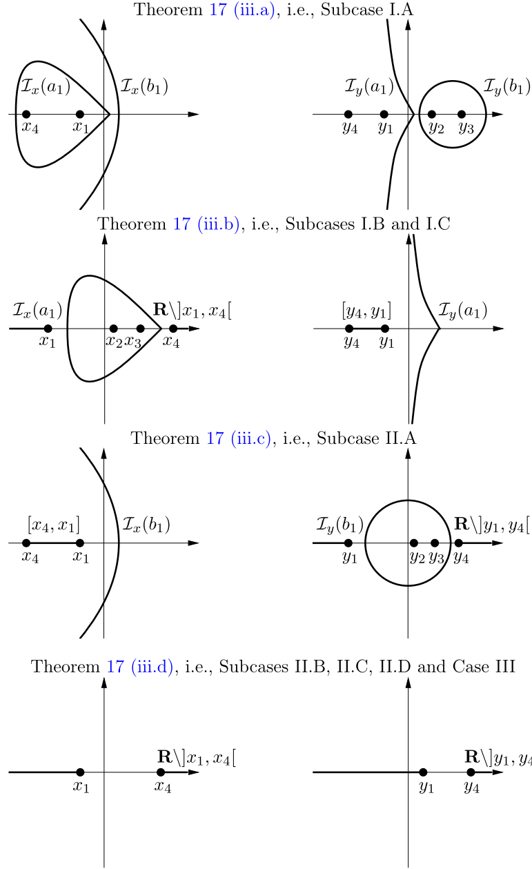
FIG. 11. — For walks pictured on Figure 17, curves where poles of the set of branches of x \mapsto Q(x, 0) and y \mapsto Q(0, y) are dense
