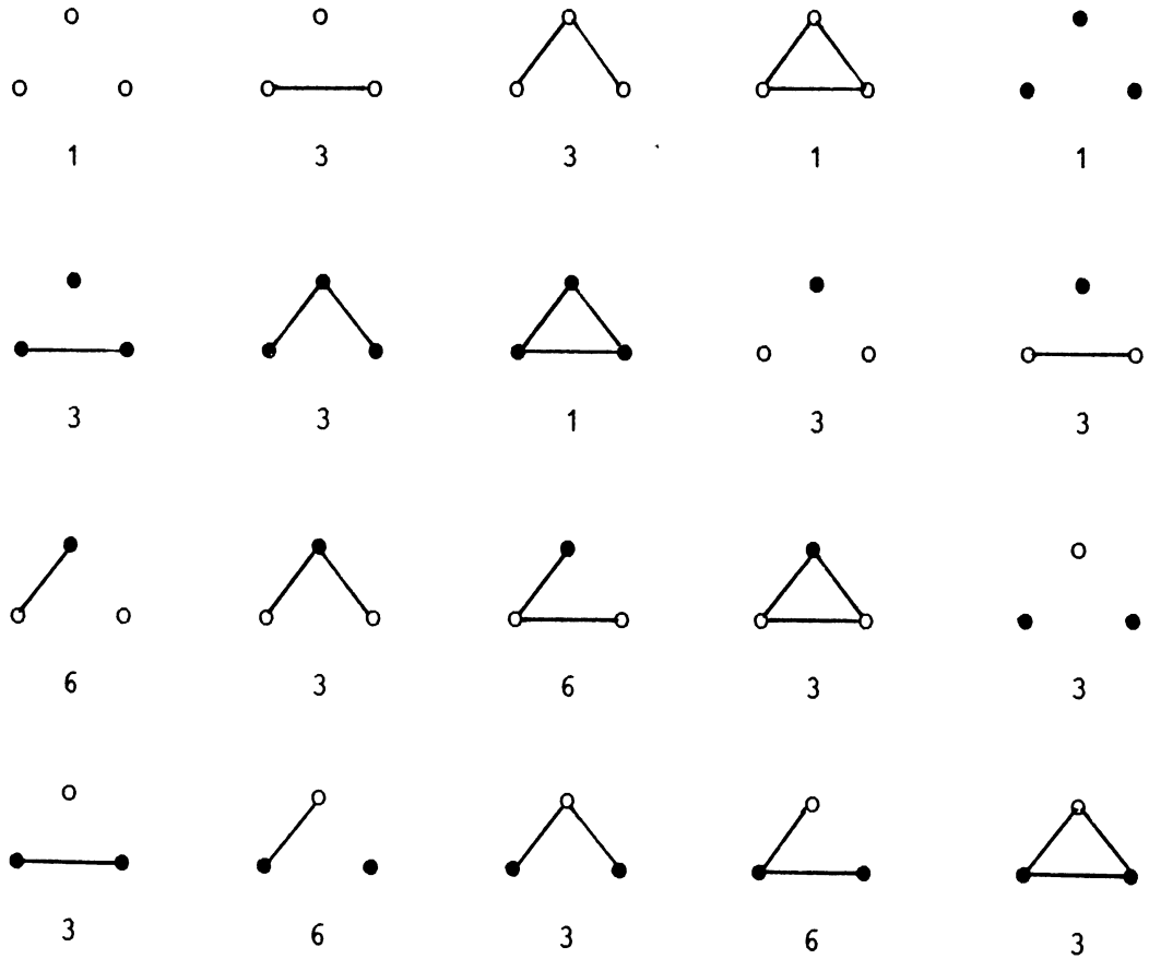
Figure 4. Graphs of order 3 with two vertex colors.
