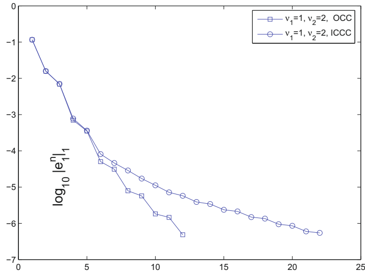
FIGURE 3. \log_{10} |e_1^n|_1 with respect to the number of iterations. The OCC method is represented by the squares, and the ICCC method is represented by the circles, with |e_1^n|_1 < 10^{-6} , \nu_1 = 1 and \nu_2 = 2 .
