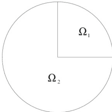
FIGURE 2. A disc decomposed into two sectors. \nu(x) = \nu_1 in \Omega_1 and \nu(x) = \nu_2 in \Omega_2 with \nu_1 \ll \nu_2 .
