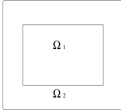
FIGURE 1. A skin fragment consisting of one cell ( \Omega_1 ) and a lipid layer ( \Omega_2 ): \nu(x) = \nu_1 inside the cell and \nu(x) = \nu_2 in the lipid layer, with \nu_1 \ll \nu_2 .
