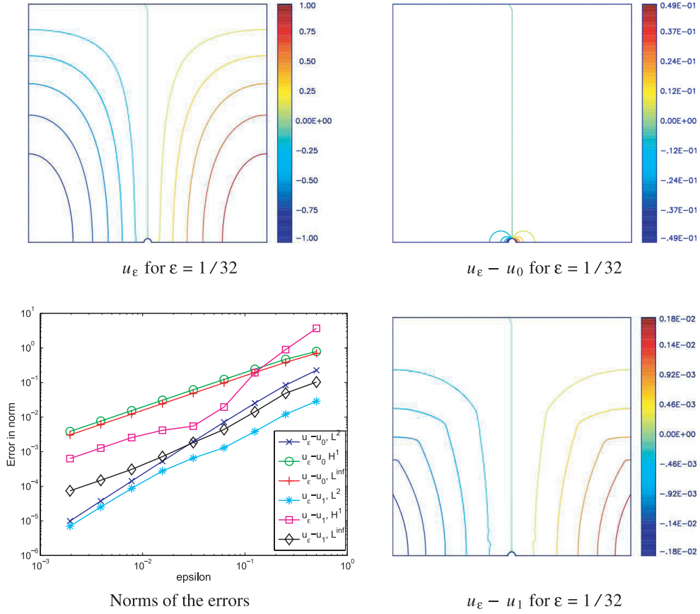
FIGURE 5. Computations for the Neumann problem (43).
