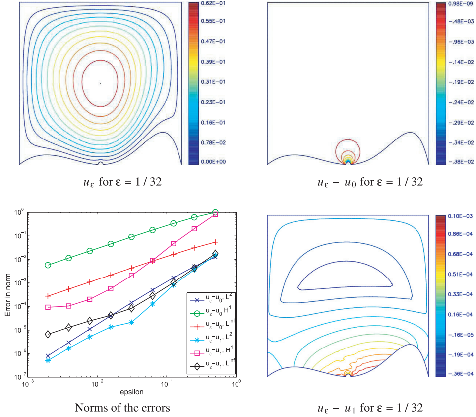
FIGURE 6. Computations for the Dirichlet problem (44).
