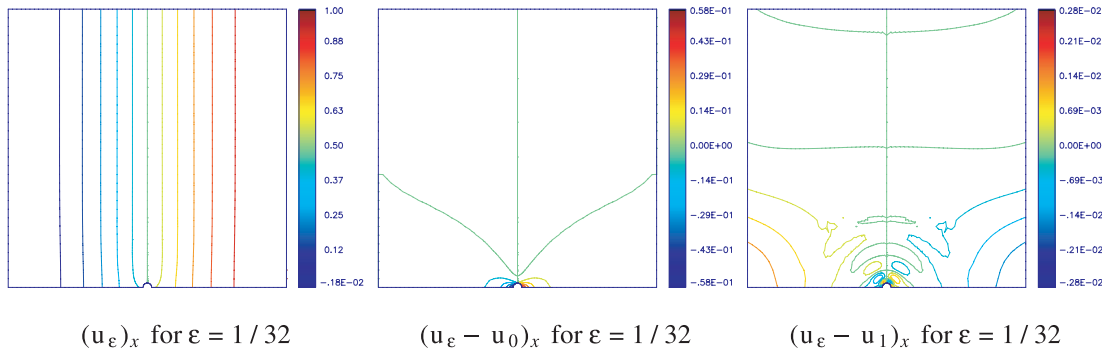
FIGURE 7. Computations for linear elasticity (45).
