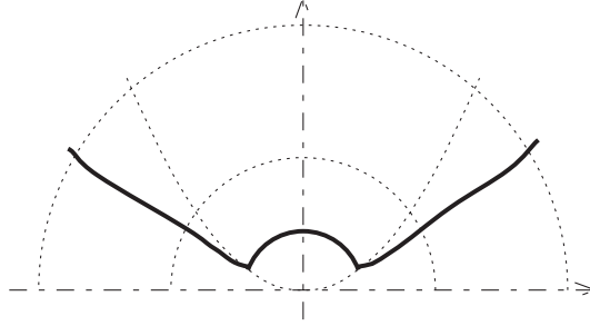
FIGURE 3. The geometrical setting of the cavity in the convex case.
