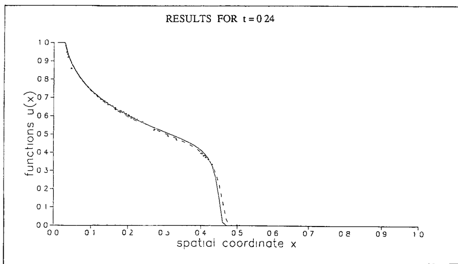
Figure 5.2. — Implicit schemes. DT = 0.008 , C.F.L. number = 1.6 ; exact solution, / computed solution by first order scheme, / second order in space first order in time, / second order in space and in time.
