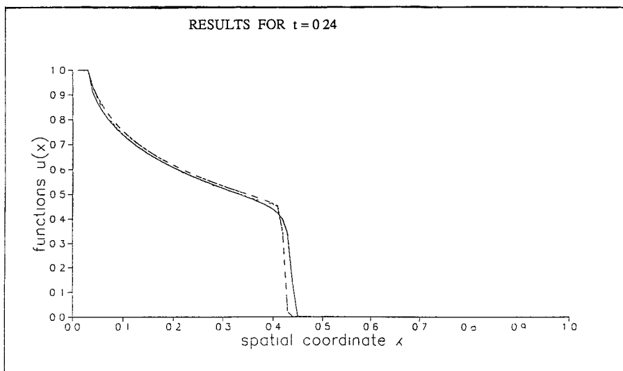
Figure 5.1. — Explicit schemes. DT = 0.03 , C.F.L. number = 0.6 ; exact solution, / computed solution by first order scheme, / second order in space first order in time, / second order in space and in time.
