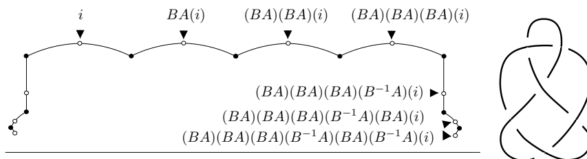
FIGURE 22. \Phi((BA)(BA)(BA)(B^{-1}A)(BA)(B^{-1}A)) = 2 and the knot \bar{6}_2
