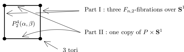
FIGURE 14. The manifold P_2^4(\alpha, \beta)
