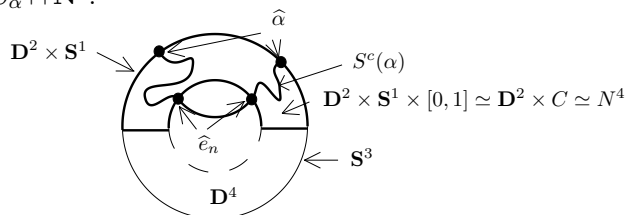
FIGURE 16. Pushing the Seifert surface in 4-ball
