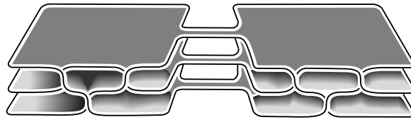
FIGURE 18. Seifert surface for a product of braids
