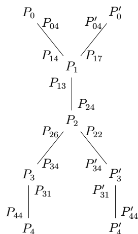
FIGURE 12.1. Assembly of the polyhedron Q from 8 chambers.
