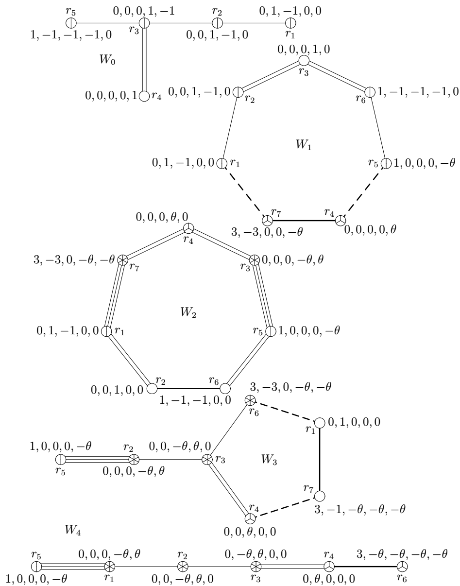
FIGURE 5.1. Simple roots for the W_j .
