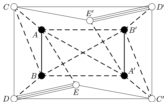
FIGURE 12.2. The polyhedron Q .
