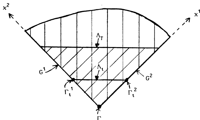
FIG. 1. — The coordinates x^3, \dots, x^{n+1} are subpressed in the figure. The domain L is shaded as ||| . The domain L_T is shaded as /// . One defines the hypersurface \Lambda_t := \{x \in L \mid T(x) = t\} with T := x^1 + x^2 being a time function.
