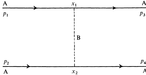
FIG. 2. — OPE graph for (AA)-scattering.
