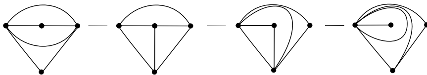
Figure 2.14. Modifying \gamma_0 to avoid a before u'
