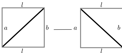
Figure 2.6. Local schematics for a cylinder flip.
