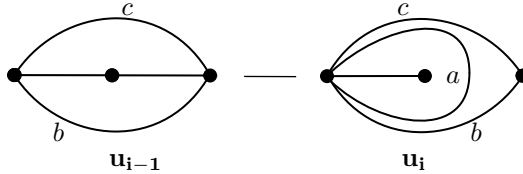
Figure 2.12. Encountering a non-maximal degree vertex on \gamma_0
