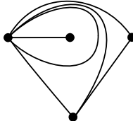
Figure 2.13. The local behavior of the triangulation u'
