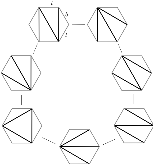
Figure 2.9. A hexagon in S , where d = b
