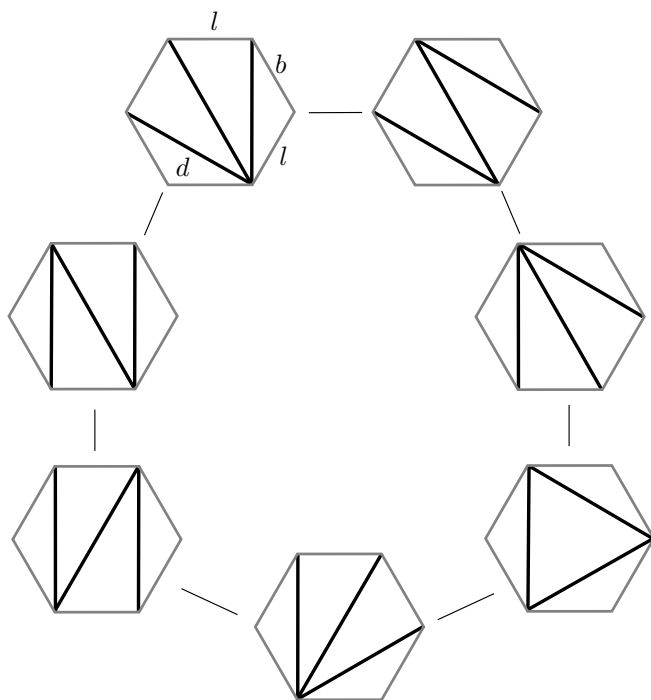
Figure 2.11. Flipping in another hexagon to get a path in \mathcal{F}(S)
