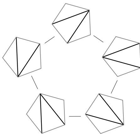
Figure 2.3. Schematics of a pentagon in the flip graph
