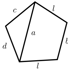
Figure 2.7. A pentagon in S , with \alpha belonging to two distinct triangles
