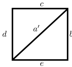
Figure 2.4. A quadrilateral in S
