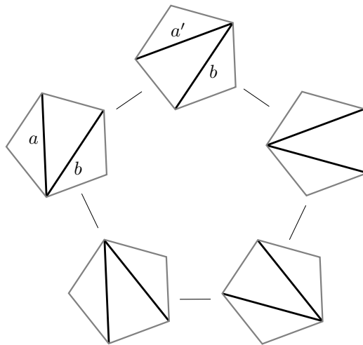
Figure 2.5. Completing edges to a pentagon in \mathcal{F}(S)
