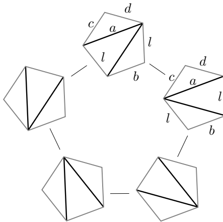
Figure 2.8. The pentagon in \mathcal{F}(S) when c, d \neq b
