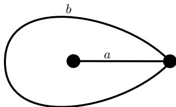
Figure 2.1. An unflippable arc of a triangulation
