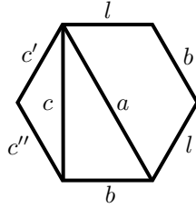
Figure 2.9. A hexagon in S , where d = b
