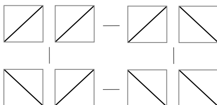
Figure 2.2. Schematics of a square in the flip graph
