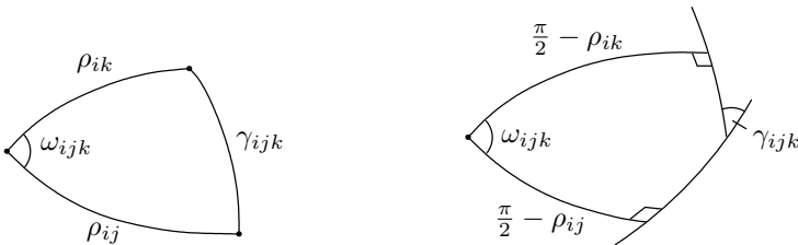
Figure 3.5. The spherical generalized polygons SP_i and SP_i^* .
