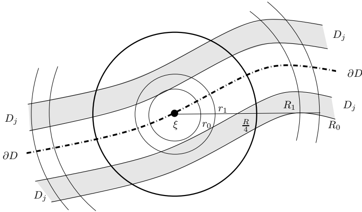
Figure 3.1. A box argument for annuli.
