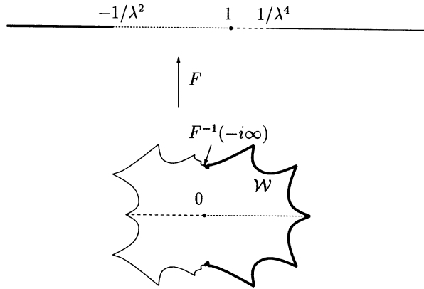
FIG. 9 - W = F^{-1}(\mathbb{C}[-1/\lambda^2, 1/\lambda^4]) .
