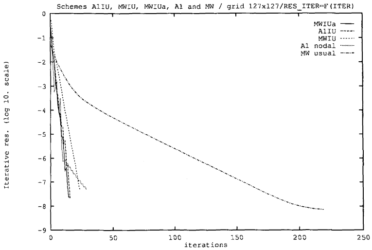
Figure 6. — Comparison of the methods MWIU, MWIUa, A1IU, A1 nodal and MW. The evolution of the residue and the iterative residue are plotted against the iterations. The grid is C_{1,6} ; \gamma = \nu = 120 , \epsilon = 2 .
