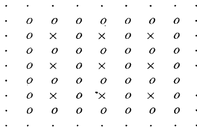
Figure 2. — Dimension 2, \Omega = ]0, 1[^2 . \times : G_H points, o : G_h \setminus G_H points.
