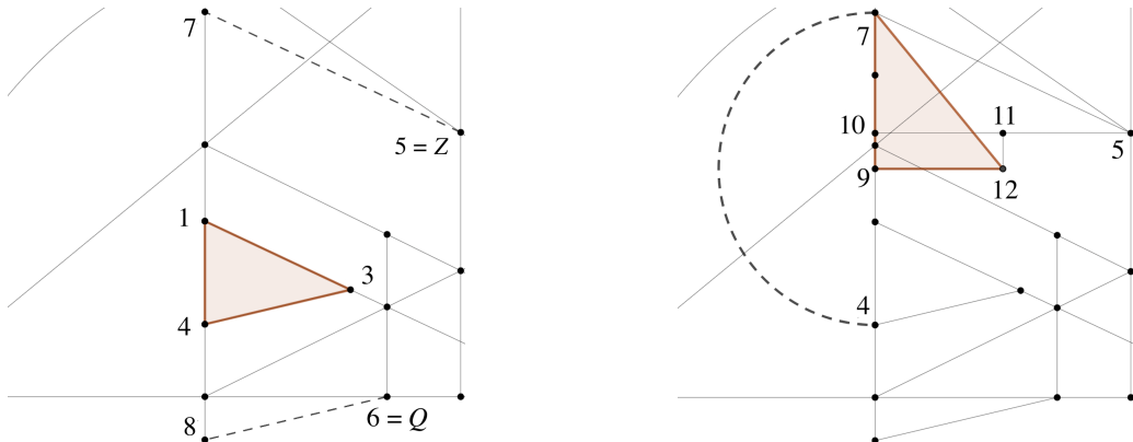
(a) Parallel lines through 5 and 6 to \overline{1,3} and \overline{4,3} meet the line (1,4) at 7 and 8, respectively.
